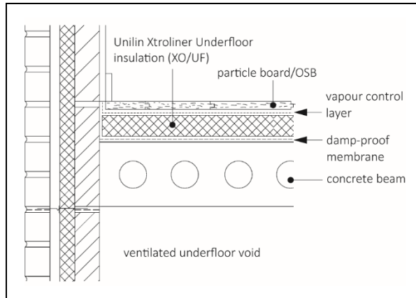
Figure 5 Suspended concrete ground floor – board overlay
