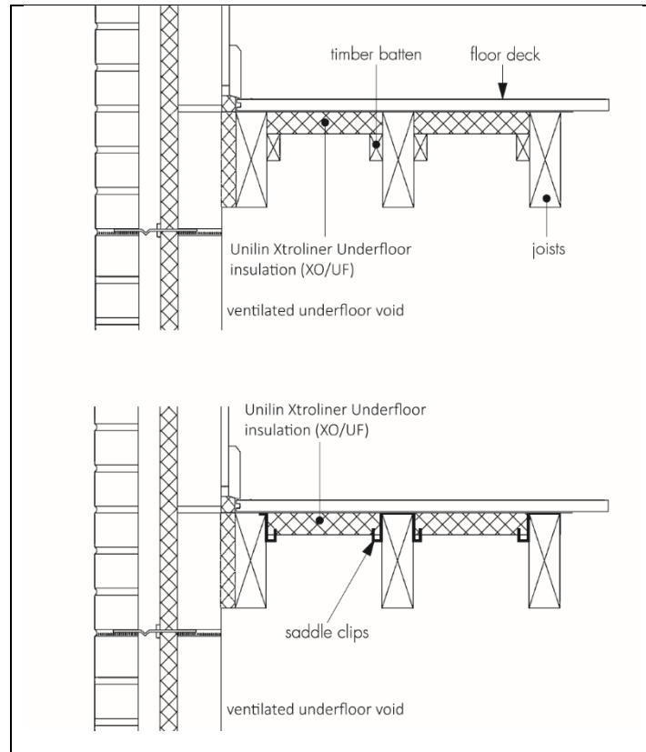
Figure 6 Suspended timber ground floors
