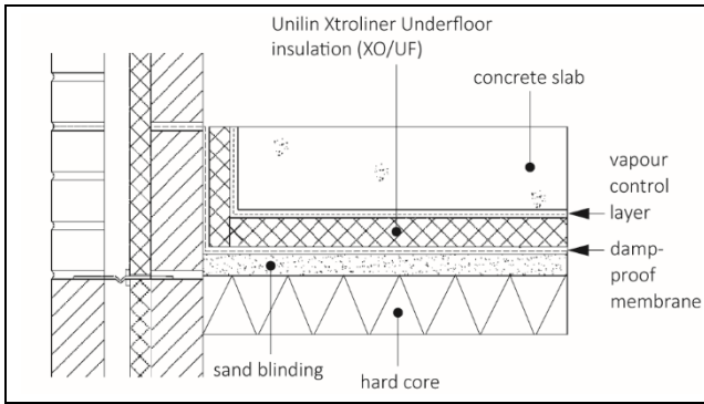
Figure 3 Ground-bearing concrete – slab overlay
