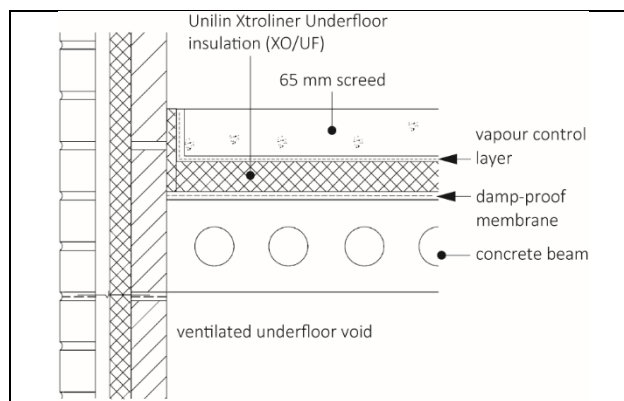
Figure 2 Suspended concrete ground floor – screed overlay
