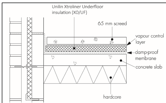
Figure 1 Ground-bearing concrete floor – screed overlay
