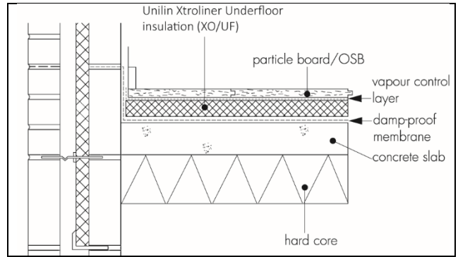
Figure 4 Ground-bearing concrete floor – board overlay
